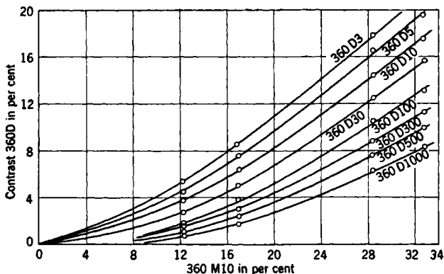
FIG. 18-56.—Decay of contrast (tube R-220) after repeated pulses in screen condensed at 35^{\circ}\text{C} and operated at 35^{\circ}\text{C} .
